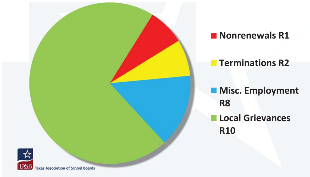
"R Number" Distribution
