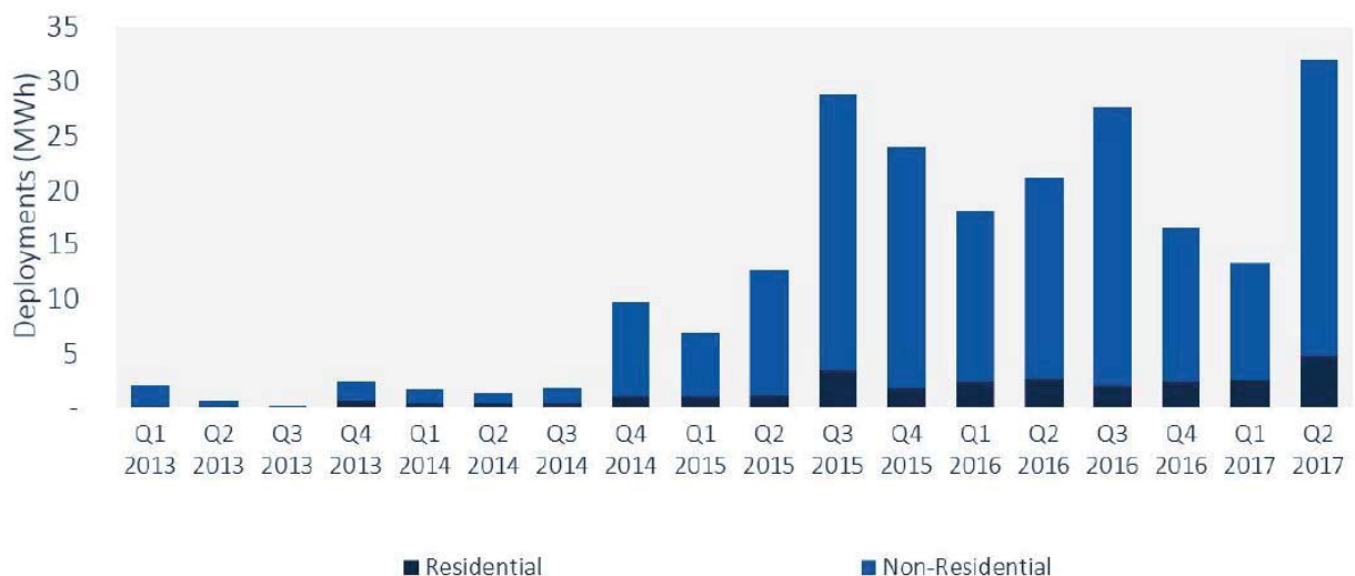
FIGURE: U.S. Behind-the-Meter Energy Storage Deployments by Segment
