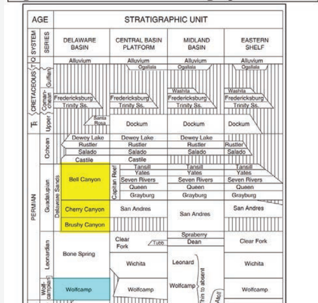
Figure 5. Permian Basin Stratigraphic Column.
