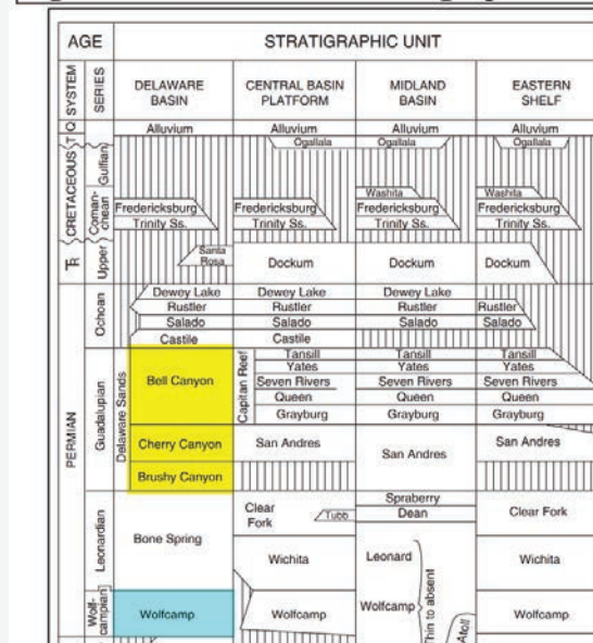
Figure 5. Permian Basin Stratigraphic Column.
