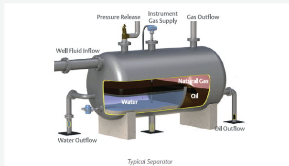
Typical Separator
