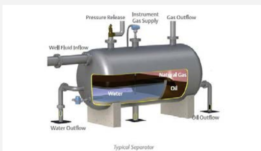
Typical Separator
